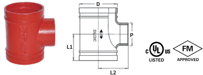
GROOVED / THREADED REDUCING TEE 레듀싱 티이 - XGQT05 / XGQT05S
