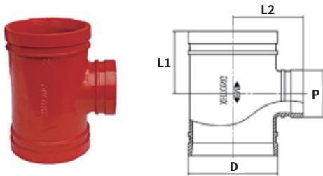
GROOVED / THREADED REDUCING TEE 레듀싱 티이 - XGQT05 / XGQT05S
